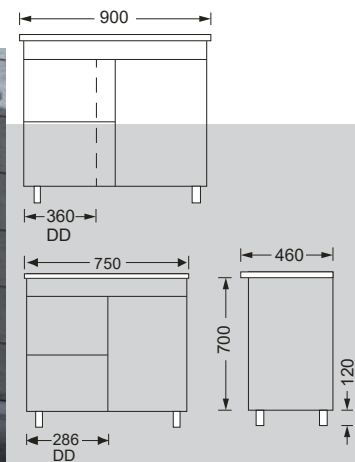
FLS 750 LH (legs) * FPS 750 (kickboard)
