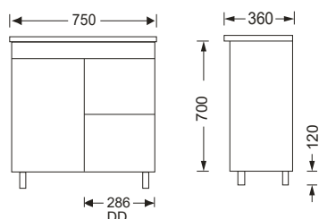
Noah FLS 7536 RH (legs) FLS 7536 LH (optional)
