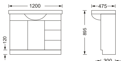
Mink RH WL 1200 (legs) WP 1200 (kickboard)
