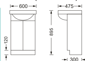
Mink WL 600 (legs) WP 600 (kickboard)
