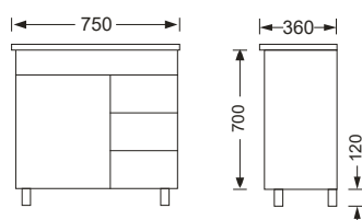
Noah WL 7536 RH (legs) WP 7536 RH (kickboard)
