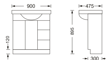
Mink RH WP 900 (kickboard)
