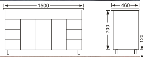
WL 1500 (legs) * WP 1500 (kickboard)
